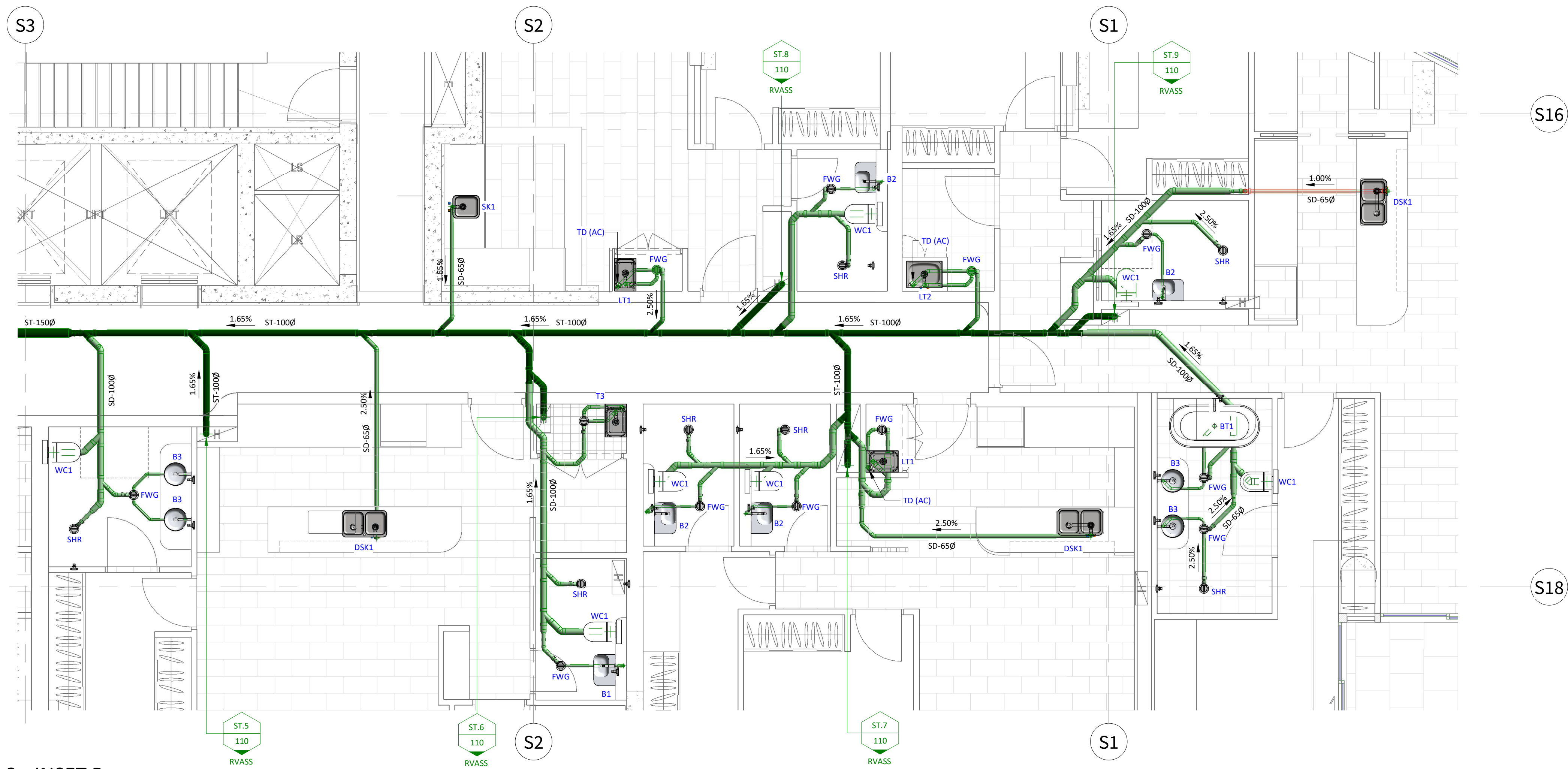
DRAINAGE PLAN - LEVEL 2 - INSET B 1 : 50
