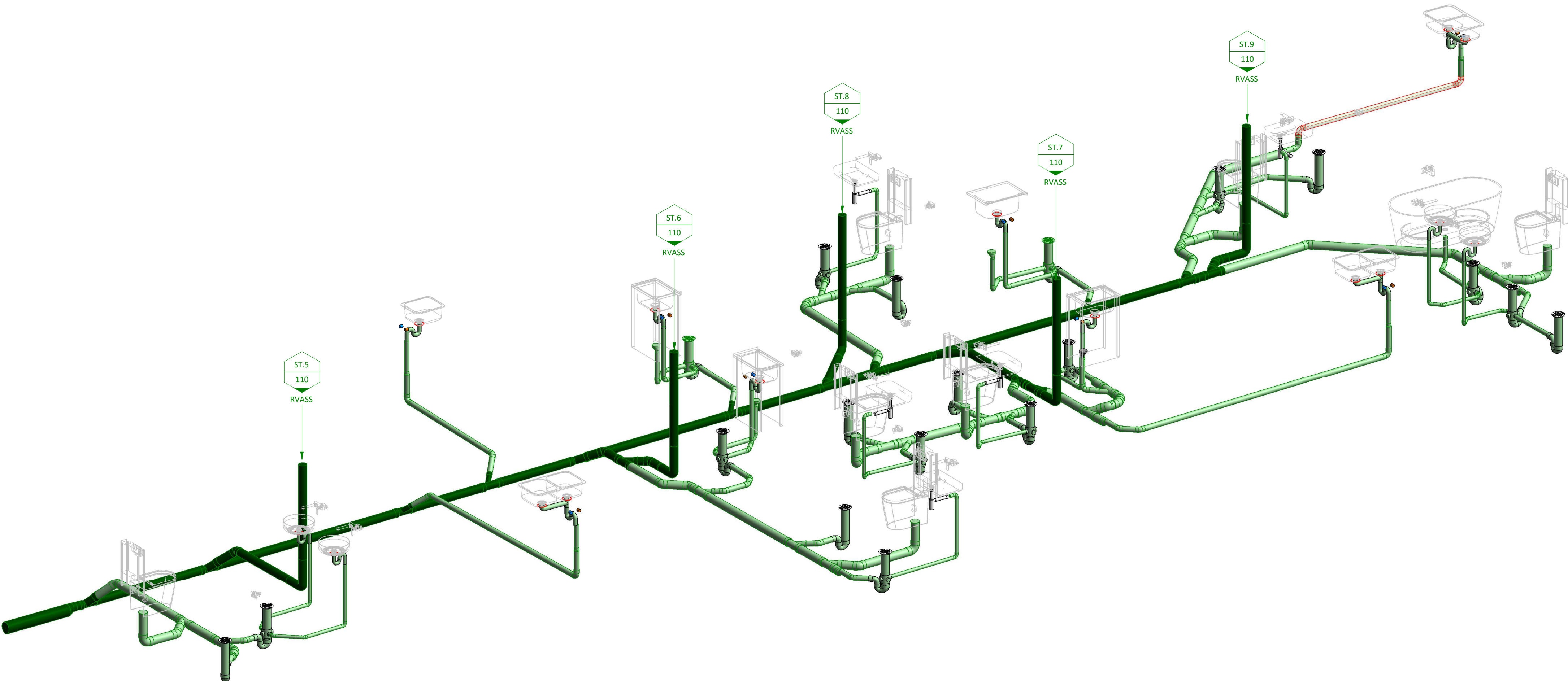
DRAINAGE PLAN - LEVEL 2 - INSET B - 3D SCHEMATIC NOT TO SCALE
